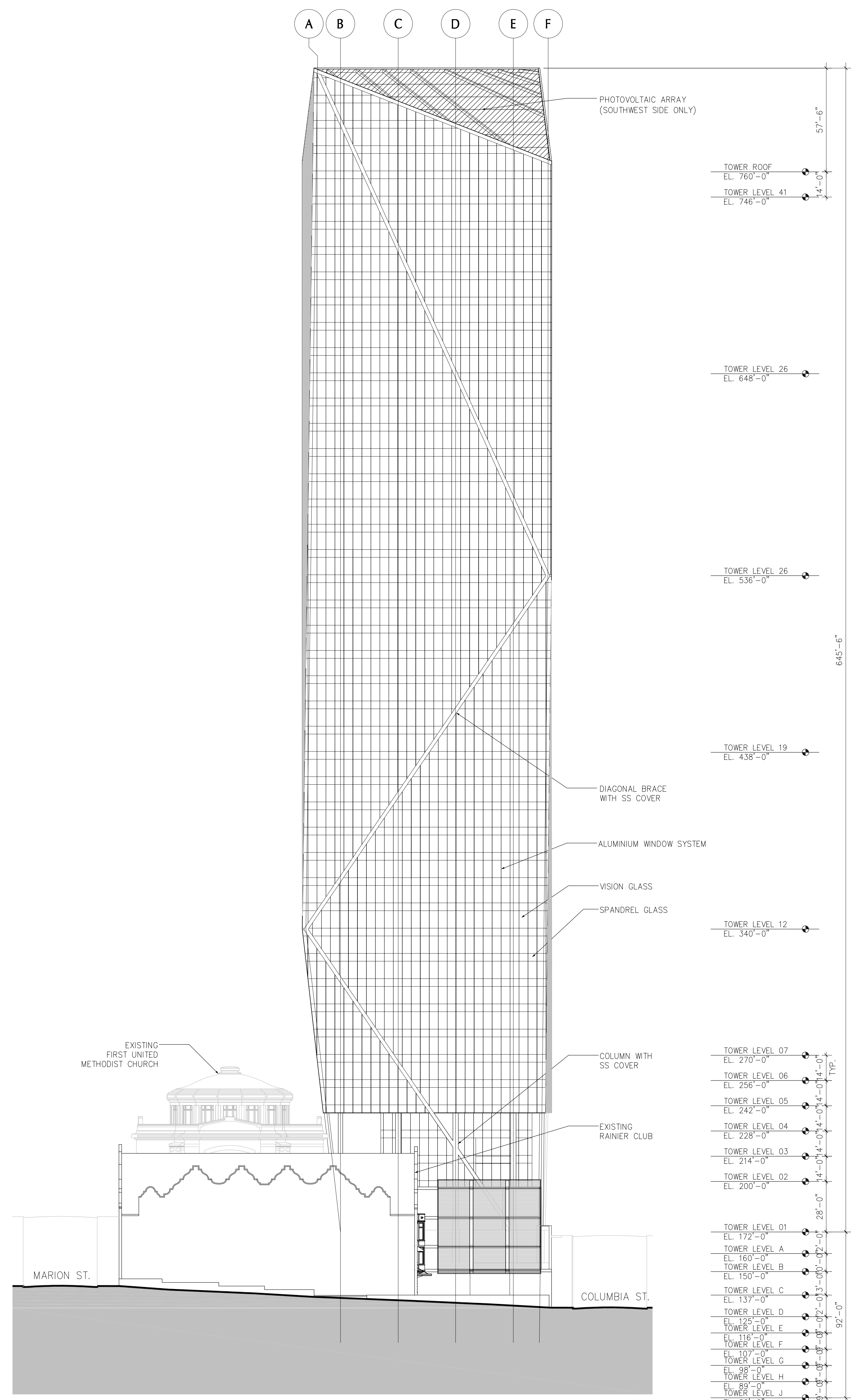
1 ELEVATION - WEST (4TH AVENUE) A3.03 SCALE: 1" = 30'
